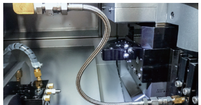
Hose mounting example (vertical tool post)
