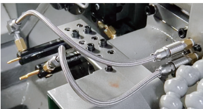
I.D. toolholder with side connection
